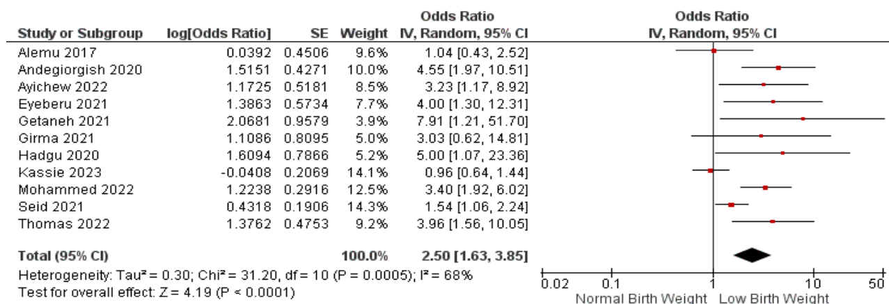
Figure 7. Forrest plot of low birth weight and neonatal mortality
